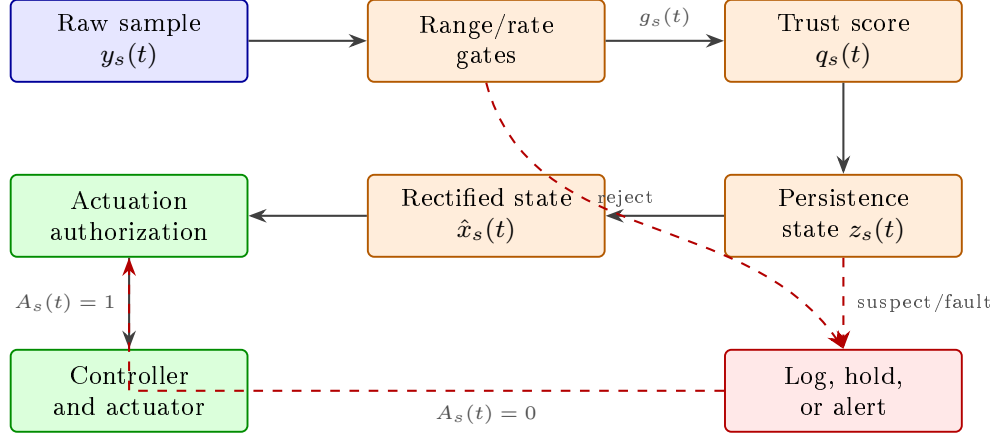
Figure 3: AASVR architecture. Measurement validation, trusted-state update, rectification, and actuation authorization are separate decisions.
