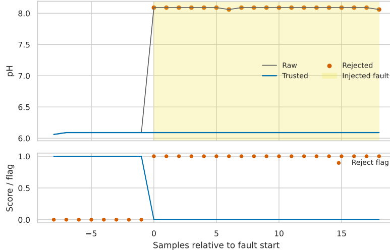
Figure 9: AASVR audit trail for a held-out pH fault replay. The shaded region is the injected fault window; rejected samples are logged without authorizing actuation.
